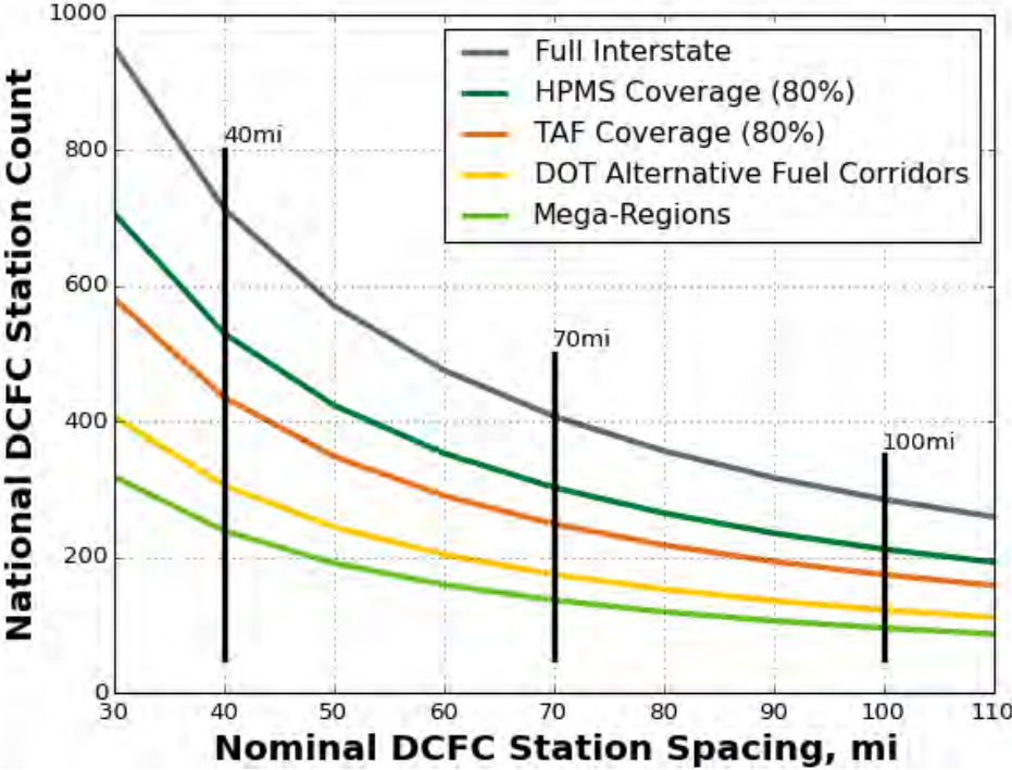
Figure 11. Nationwide DCFC station counts to cover corridors as a function of station spacing for different scenarios.
