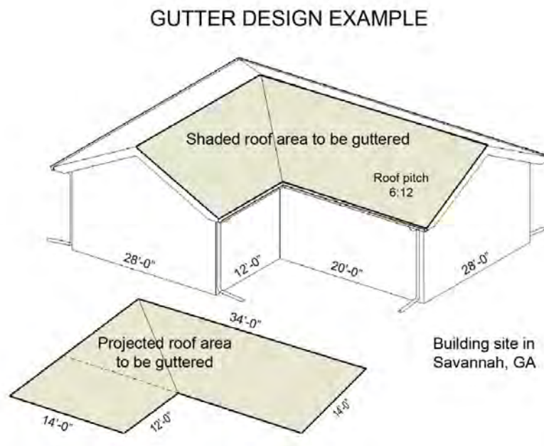
Figure 4–9: Gutter Design Example
