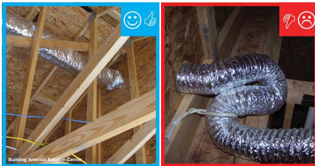
Good and bad duct examples. Good: straight, supported exhaust duct venting to outdoors. Bad: kinked duct with very restricted flow and compromised performance.
