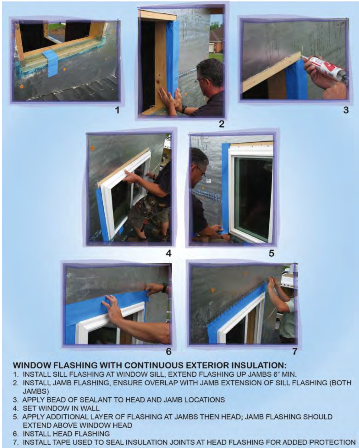
Figure 4-13: Window Flashing Sequence on a Wall With Exterior Foam Insulation
