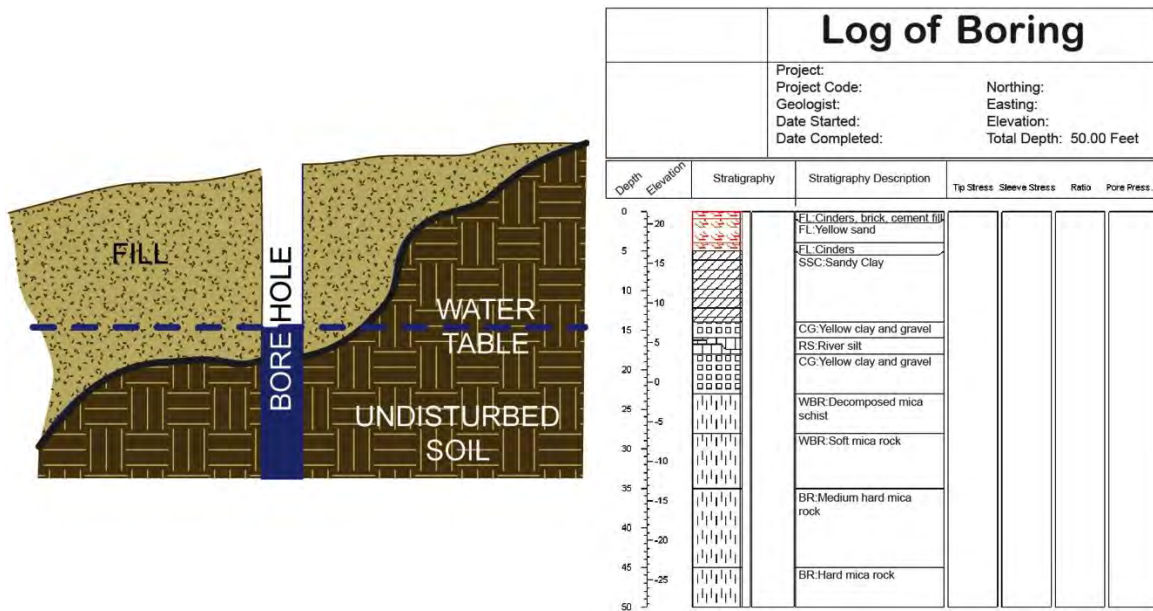
Figure 3-1: Bore Hole and Bore Log
