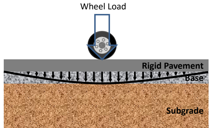
Figure 4. Illustrations. How rigid pavements and flexible pavements transfer applied loads to the layers beneath.
