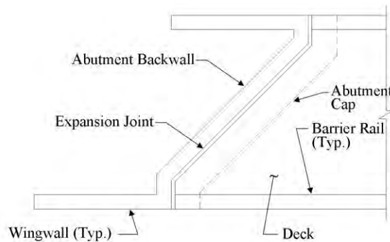
Figure 9 Breakback detailing to eliminate skew effects associated with detailing acute corners at ends of skewed deck slab (8).
