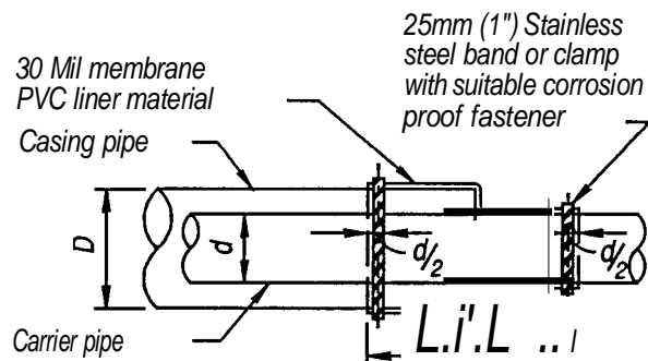
END SEAL DETAIL FOR CASING PIPE
