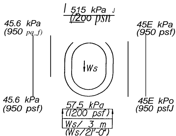
LOADING DIAGRAM
