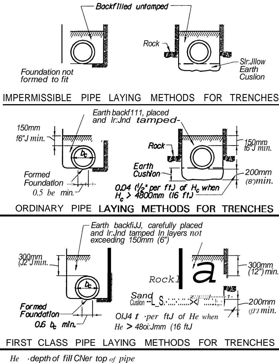
Figure 3-1. Trench bedding conditions
