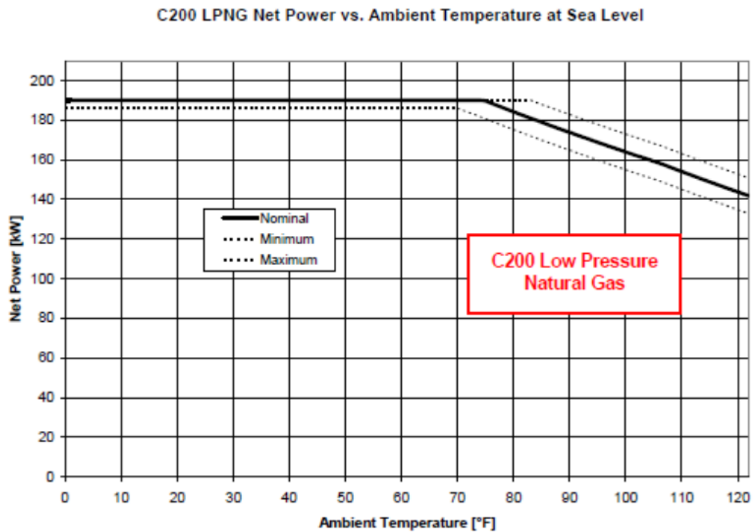
Figure 4. Temperature Effect on Power, Capstone C200-LP
