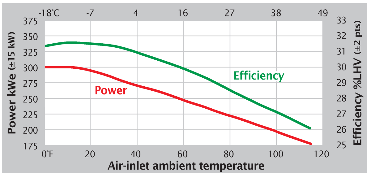
Figure 6. Temperature Effect on Power and Efficiency, FlexEnergy MT250
