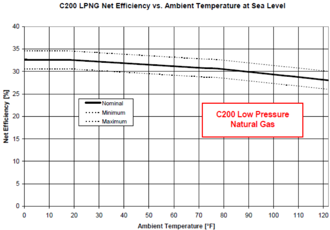
Figure 5. Temperature Effect on Efficiency, Capstone C200-LP
