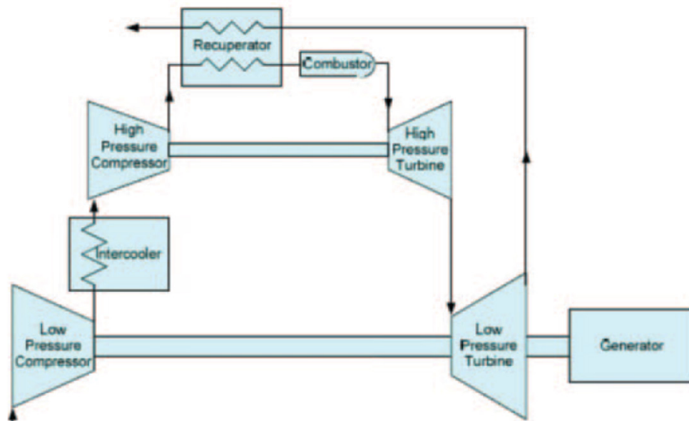
Figure 8. Capstone C370 Two-shaft High Efficiency Turbine Design
