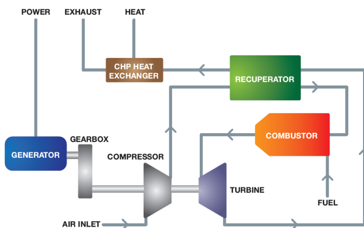
Figure 1. Microturbine-based CHP System Schematic
