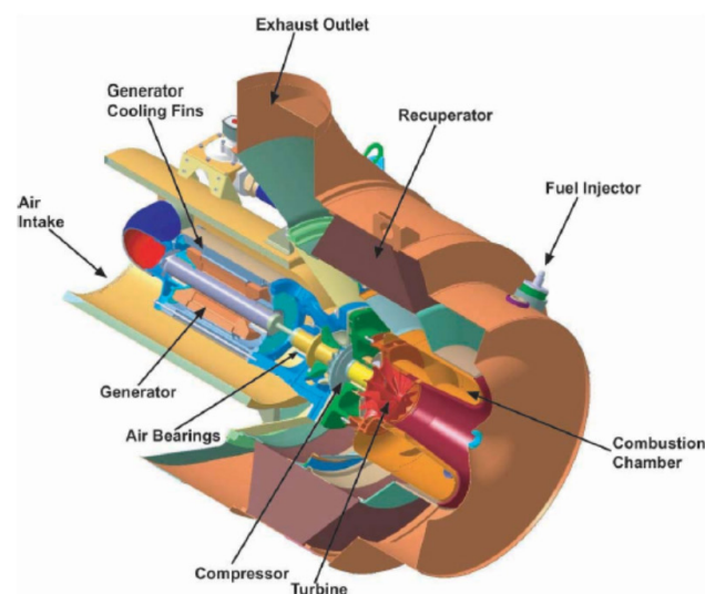
Figure 2. Compact Microturbine Design
