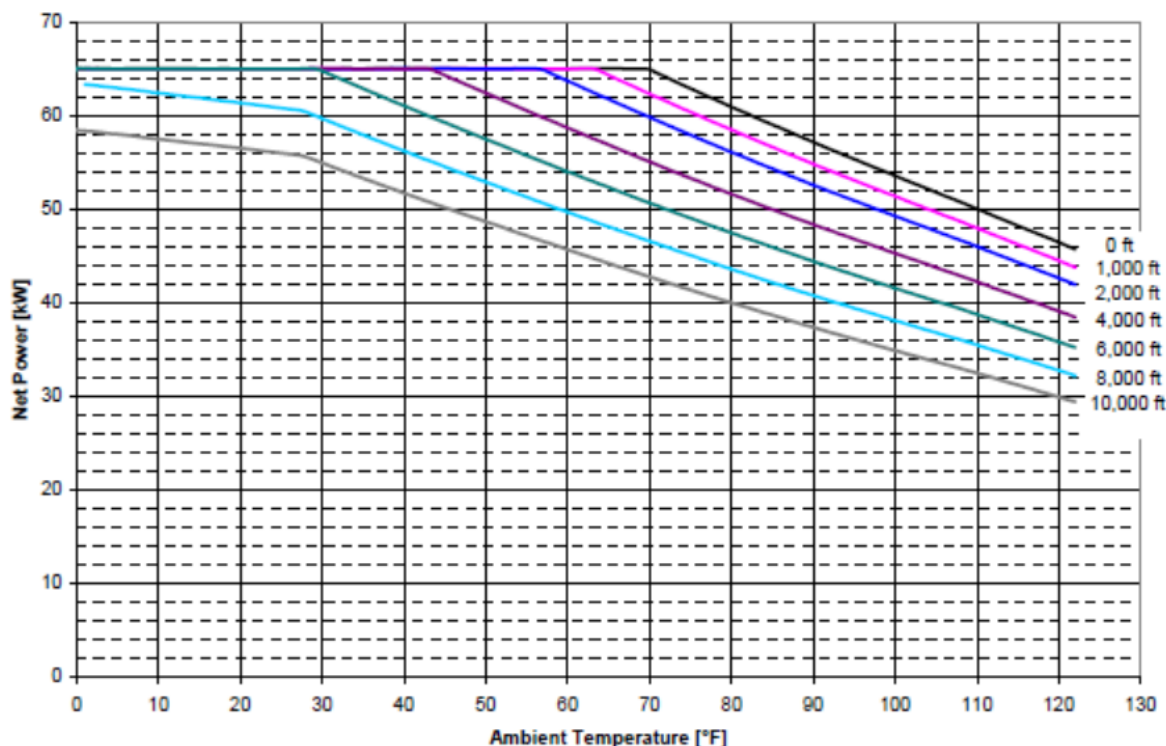
Figure 7. Ambient Elevation vs. Temperature Derating, Capstone C65
