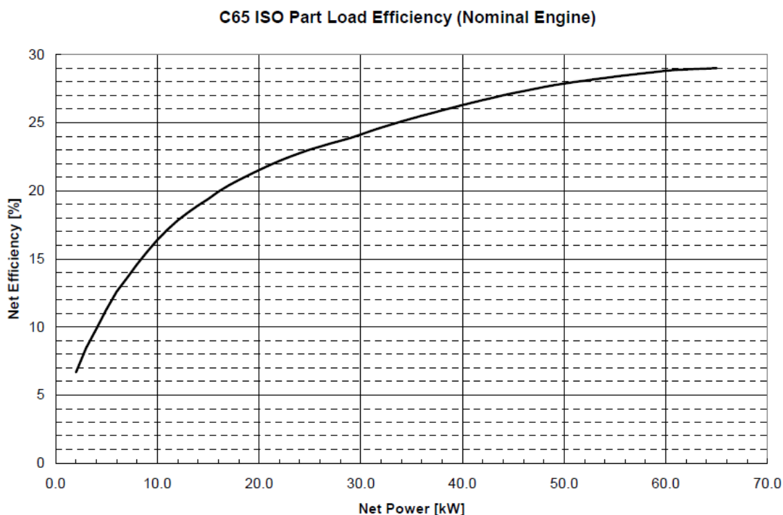
Figure 3. Part Load Efficiency at ISO Conditions, Capstone C65
