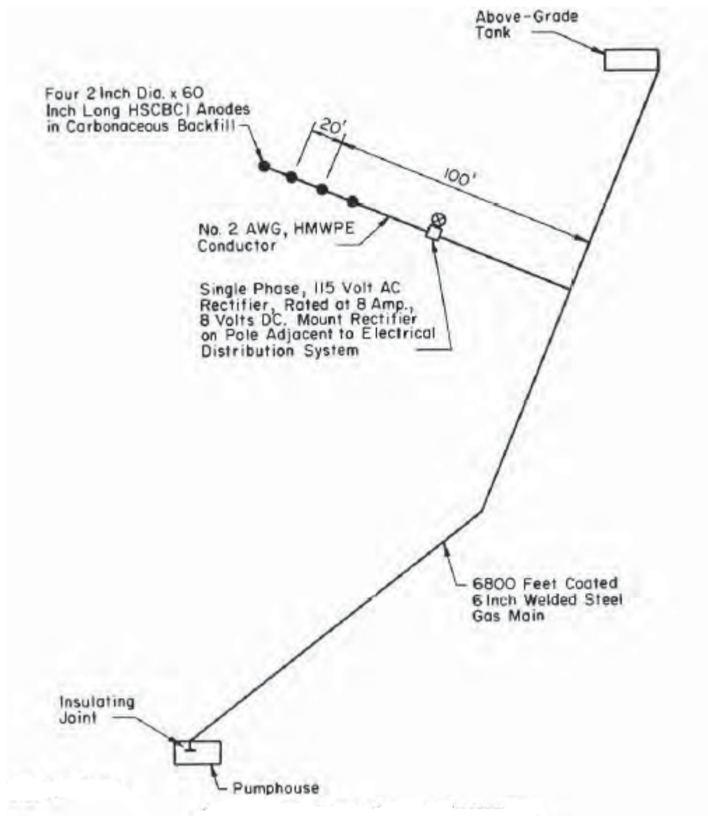
Figure 5-1 Cathodic protection system for gas main
