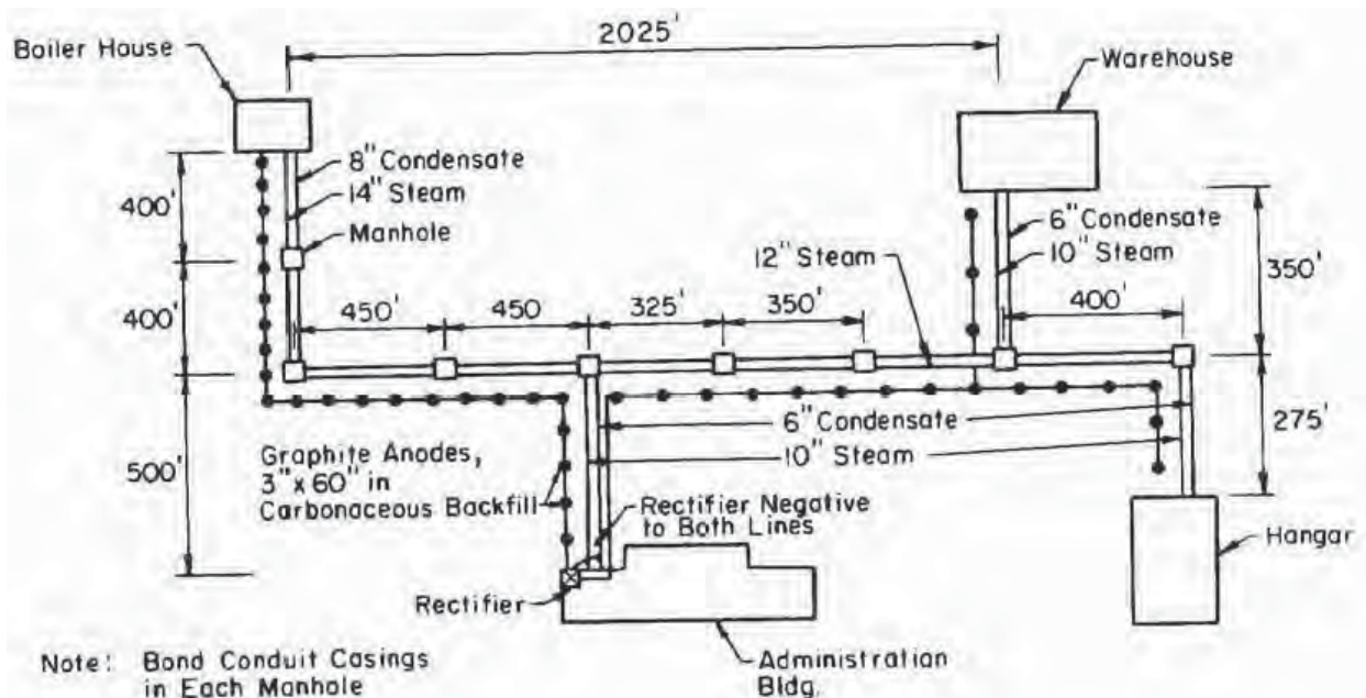
Figure 5-2 Heating Distribution System
