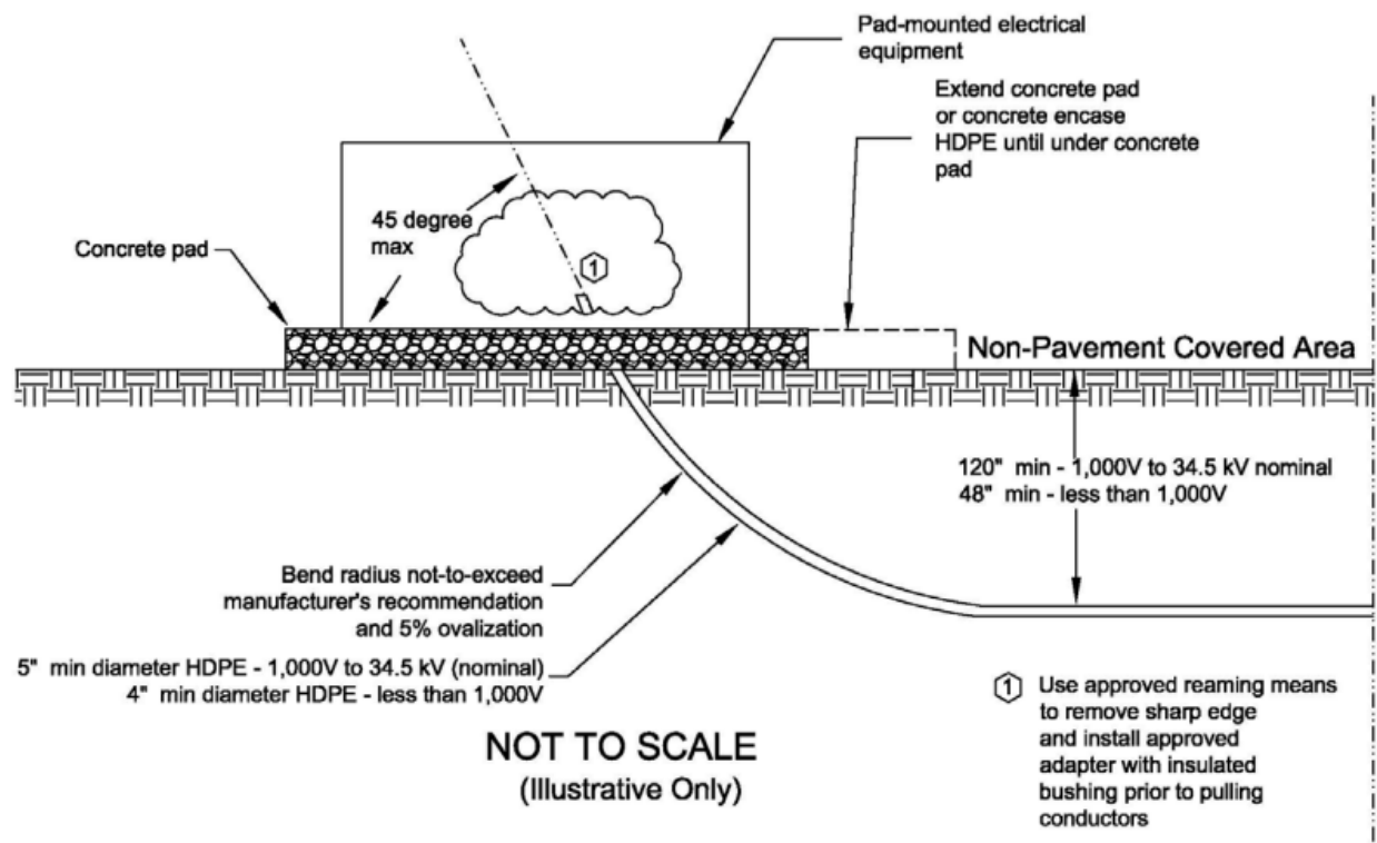
Figure A-5. Non-Pavement Covered Area to Electrical Equipment Transition – HDPE Conduit (20°–45°)
