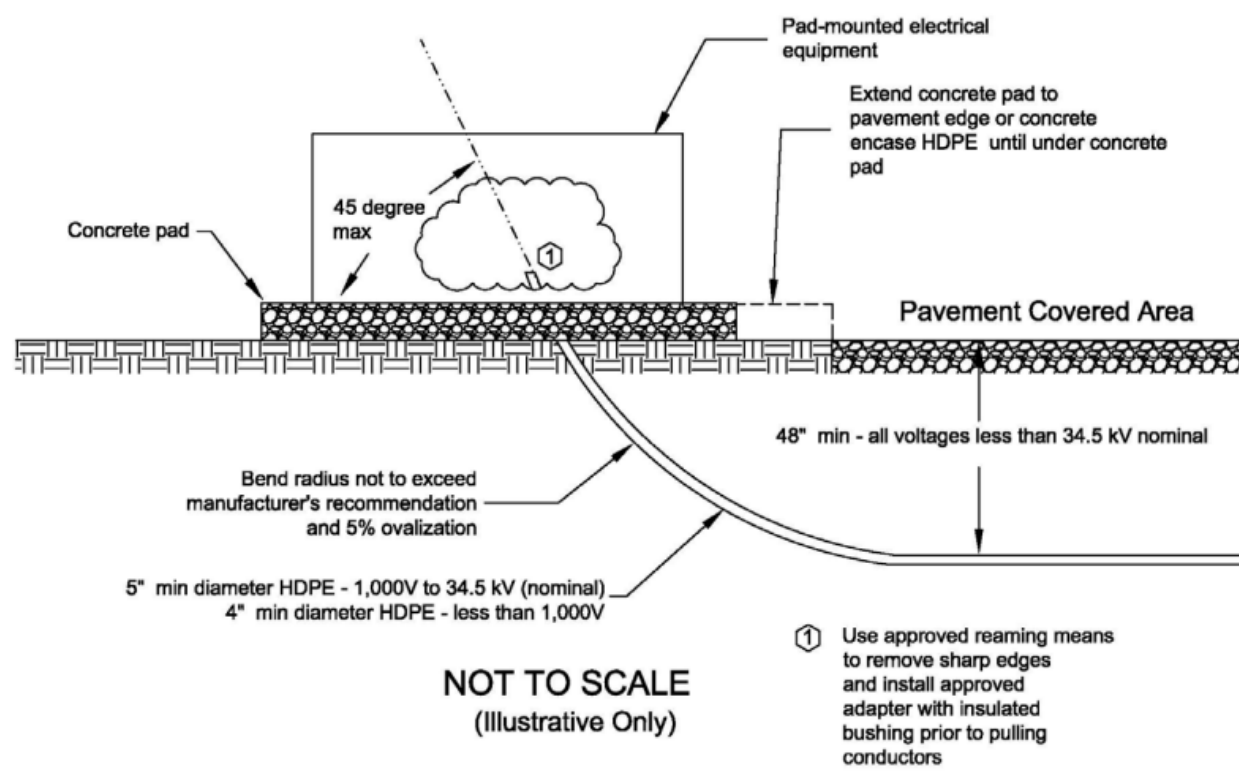
Figure A-3. Pavement Covered Area to Electrical Equipment Transition – HDPE Conduit (20°–45°)
