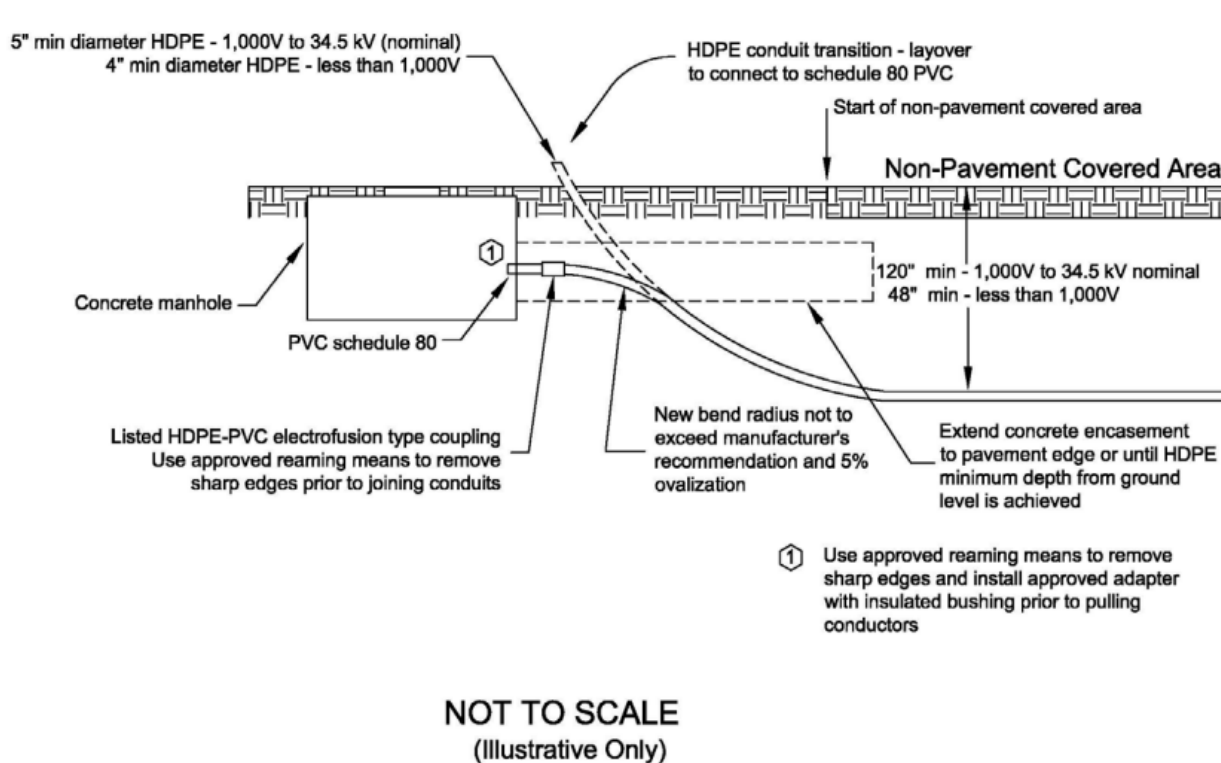
Figure A-9. HDPE-to-Manhole Pavement Covered Area Transition
