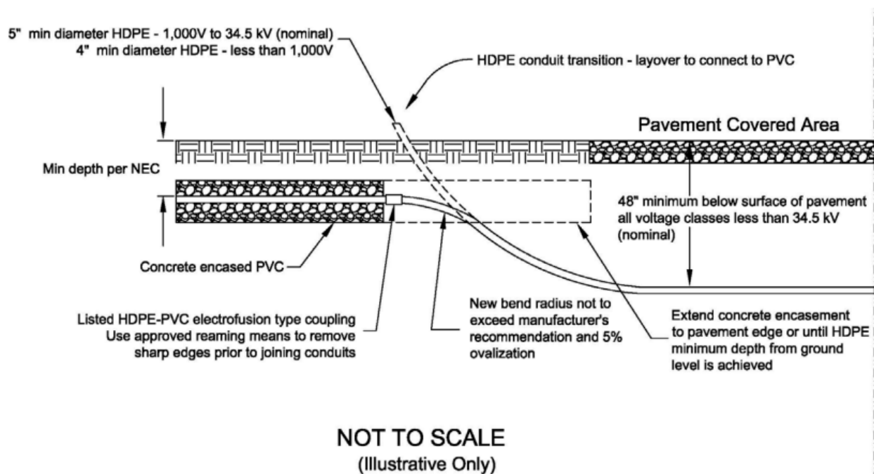
Figure A-6. HDPE-to-PVC Pavement Covered Area Concrete Ductbank Transition
