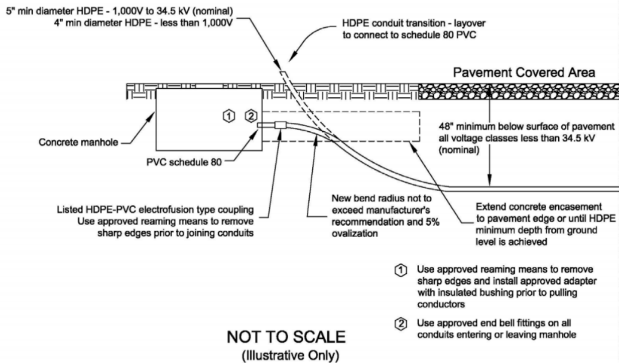
Figure A-8. HDPE-to-Manhole Pavement Covered Area Transition
