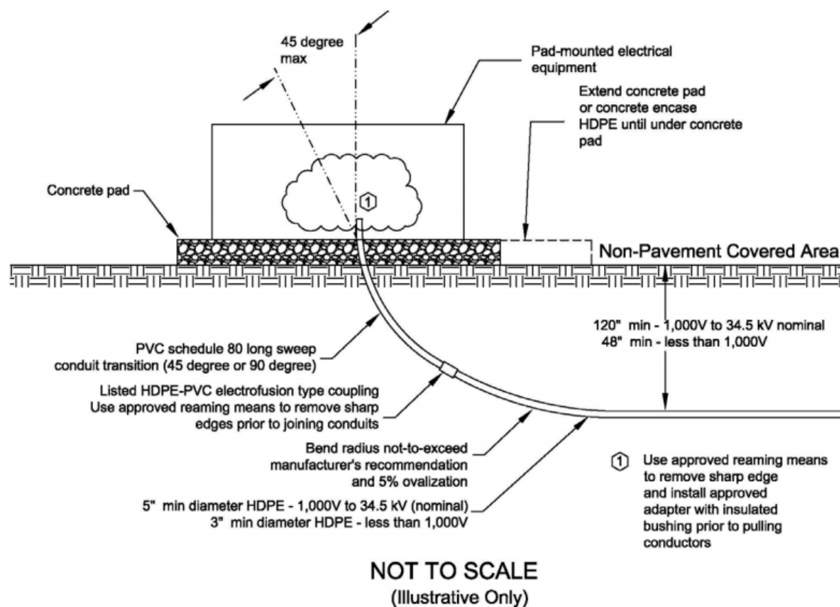
Figure A-4. Non-Pavement Covered Area to Electrical Equipment Transition – Rigid Conduit (45°–90°)
