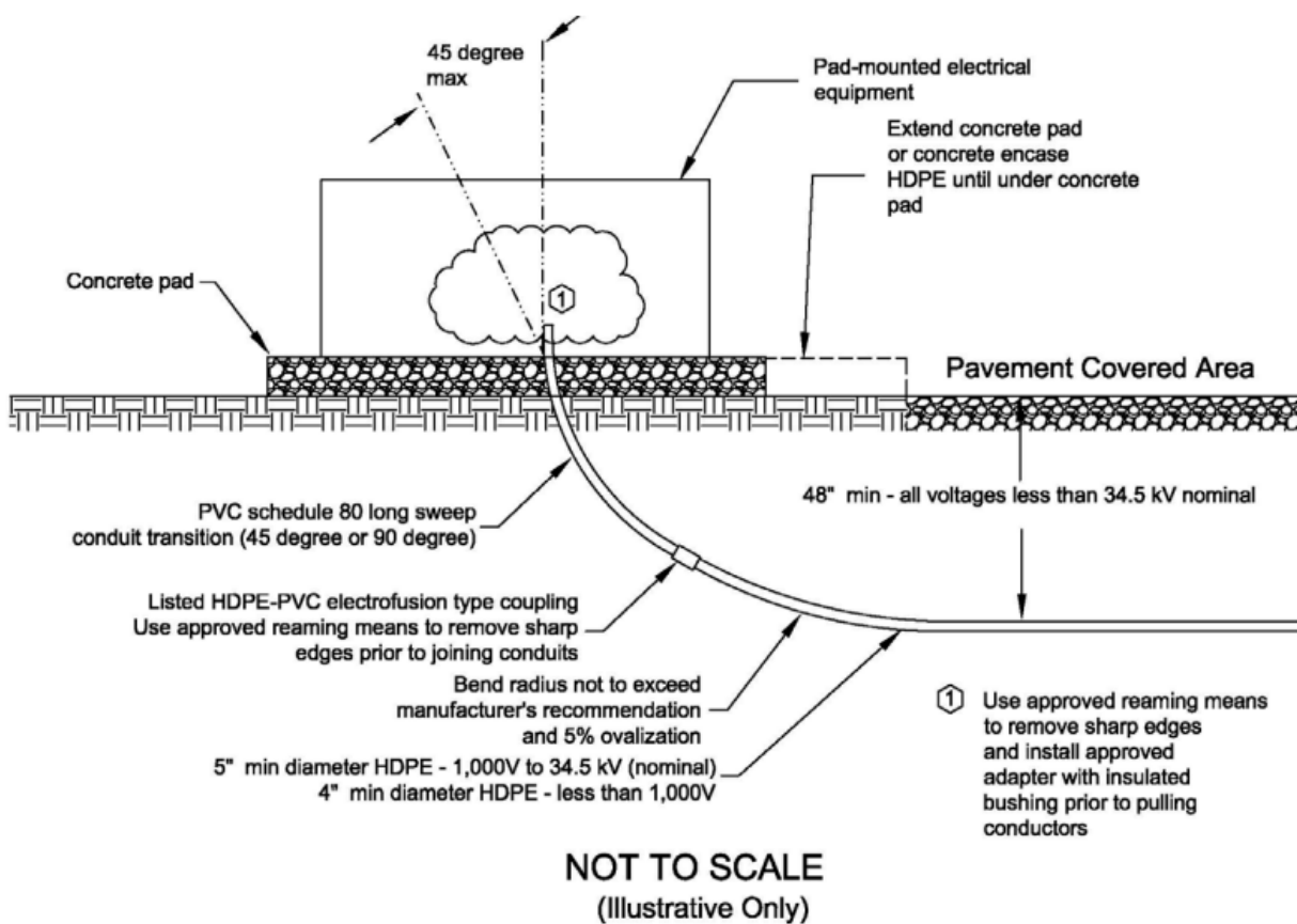
Figure A-2. Pavement Covered Area to Electrical Equipment Transition – Rigid Conduit (45°–90°)
