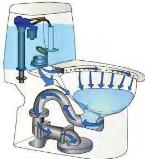
Figure 54 — Siphon jet bowl.
