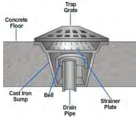
Figure 28 – Drain without a water seal.
