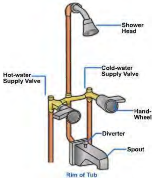
Figure 21 – Bathtub and shower piping arrangement.
