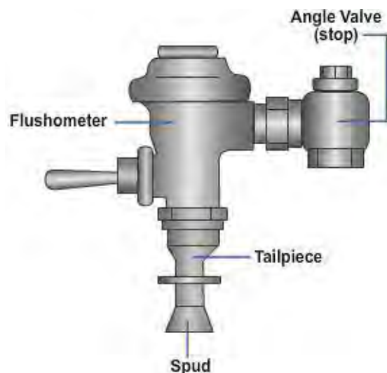
Figure 56 – Flushometer.
