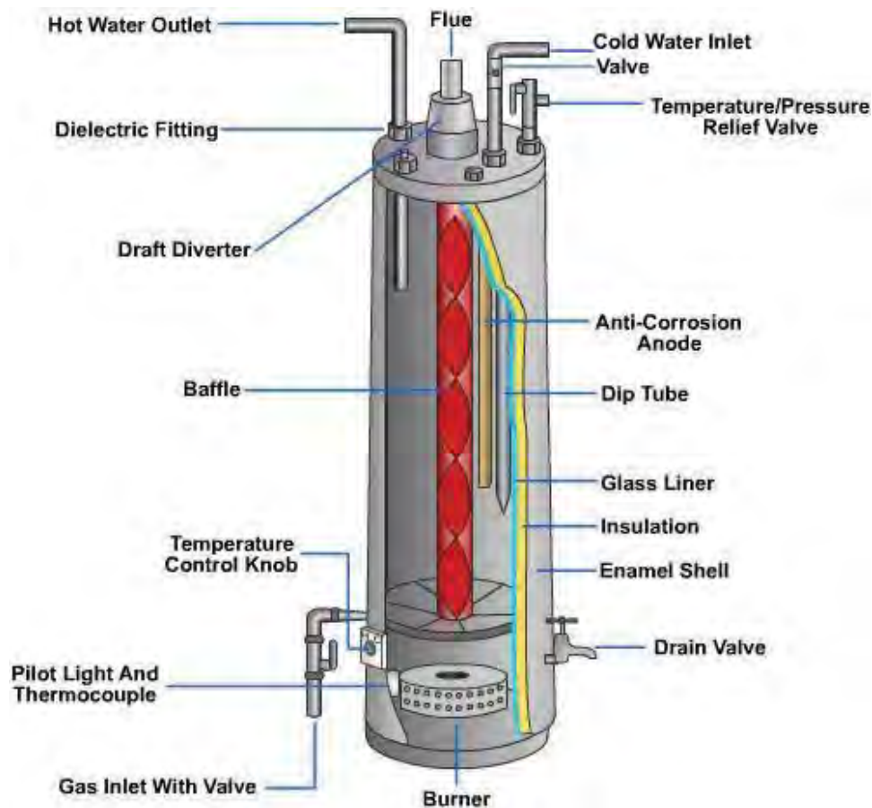
Figure 51 – Gas water heater components.
