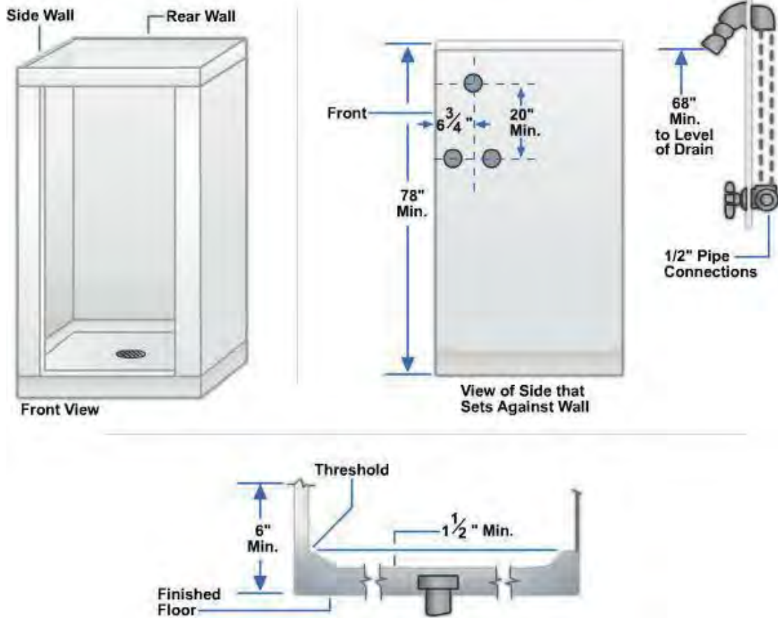
Figure 24 – Shower stalls and sections.
