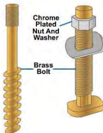
Figure 58 – Water closet bolts and screws.
