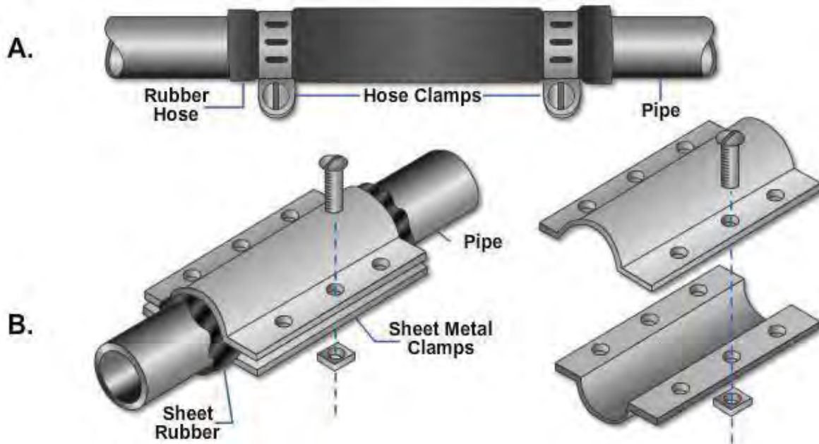
Figure 34 – Temporary types of repairs of a leaky pipe.
