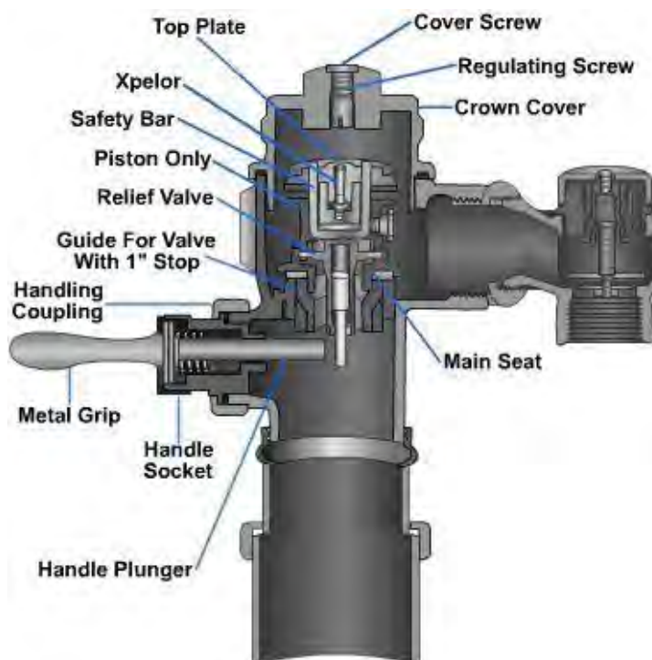
Figure 9 – Piston type of flushing valve.
