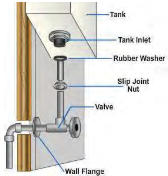
Figure 6 – Closet tank water supply line.
