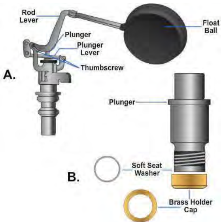
Figure 37 — A. Ball cock. B. Plunger need washer and cap.
