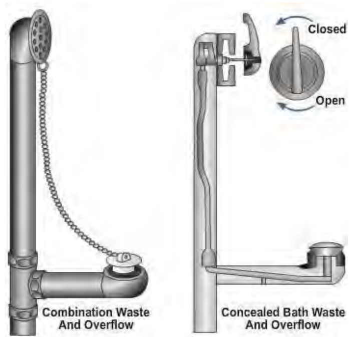
Figure 19 - Bathtub combination waste and overflow.
