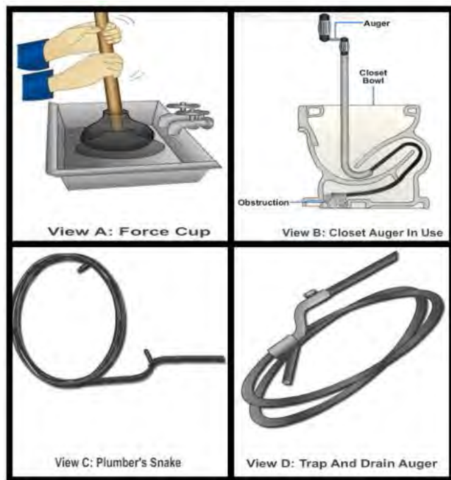
Figure 49 – Tools for clearing stoppages in plumbing fixtures.
