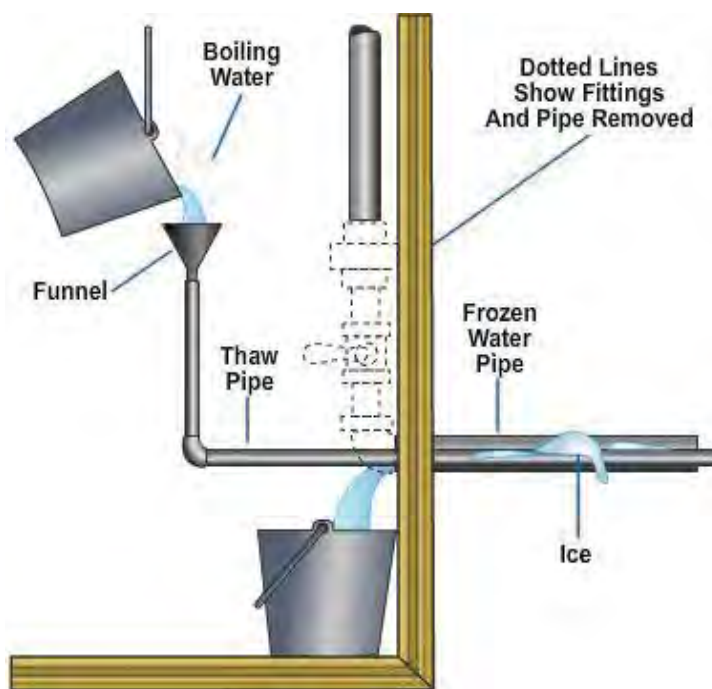
Figure 29 – Thawing an underground or otherwise inaccessible pipe.
