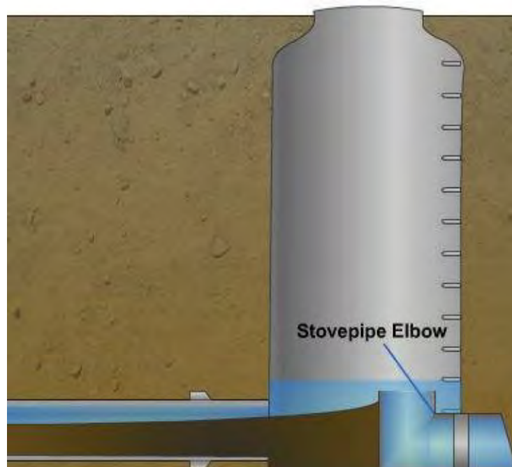
Figure 46 – Sand trap.
