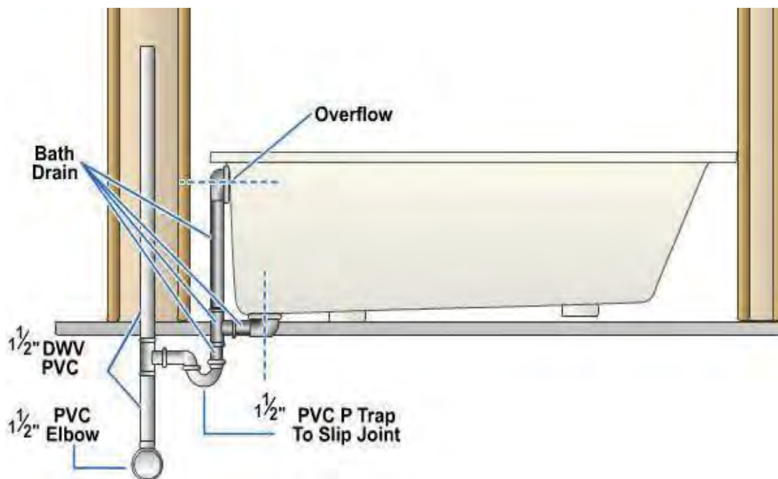
Figure 20 – Tub waste hookup.
