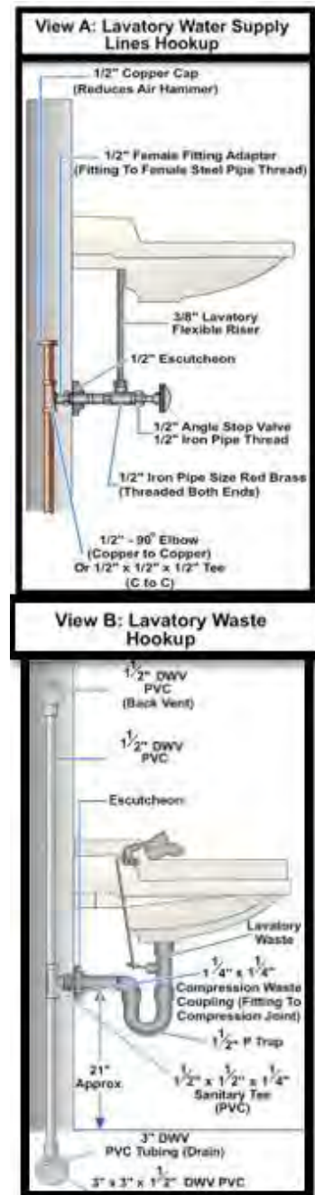
Figure 15 – Lavatory water supply and waste hookups.
