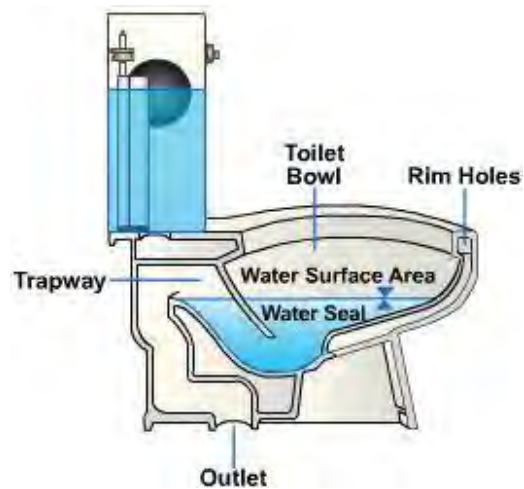
Figure 55 – Common wash down bowl.
