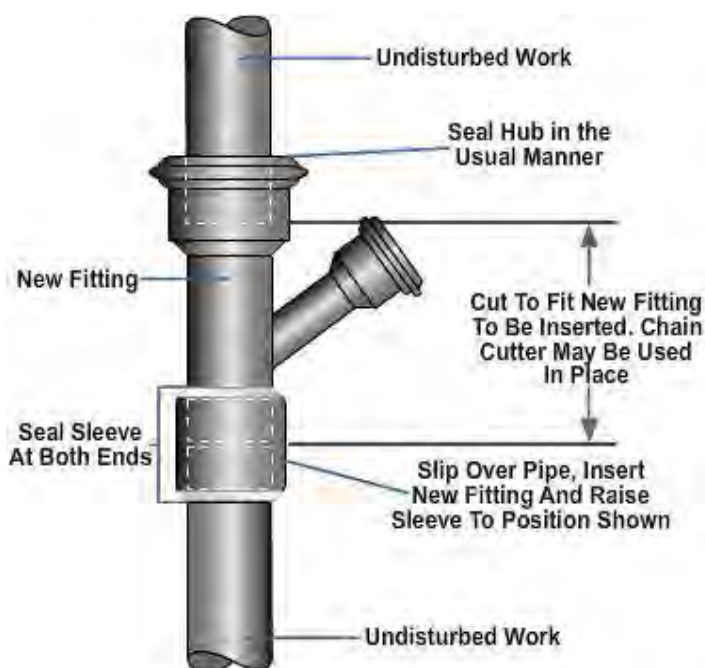
Figure 32 – Installing a fitting in a restricted space.
