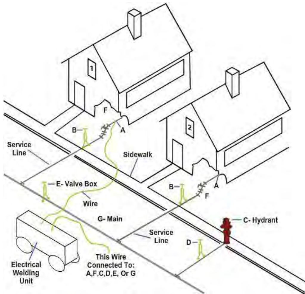
Figure 30 — Connection points for thawing frozen service lines.
