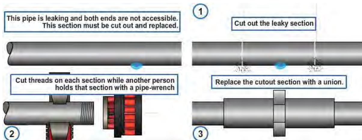
Figure 31 – Replacing a leaking section of pipe.
