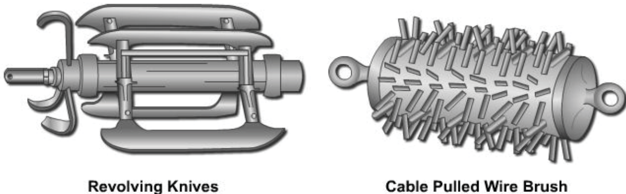
Figure 47 – Turbine-driven tools.
