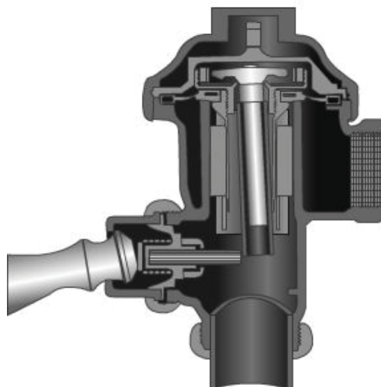
Figure 8 – Diaphragm type of flushing valve.
