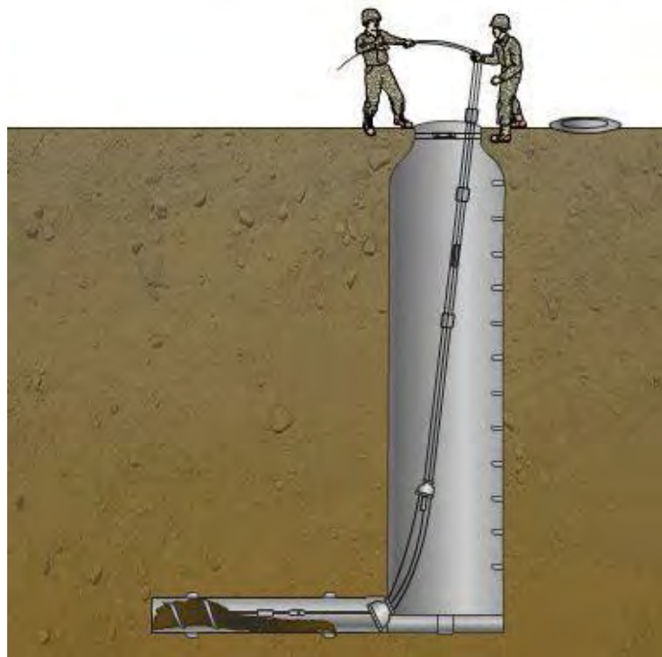
Figure 45 – Root removal by steel rod and auger, manual operation.
