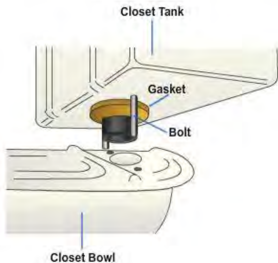
Figure 5 – Mounting a close coupled tank.
