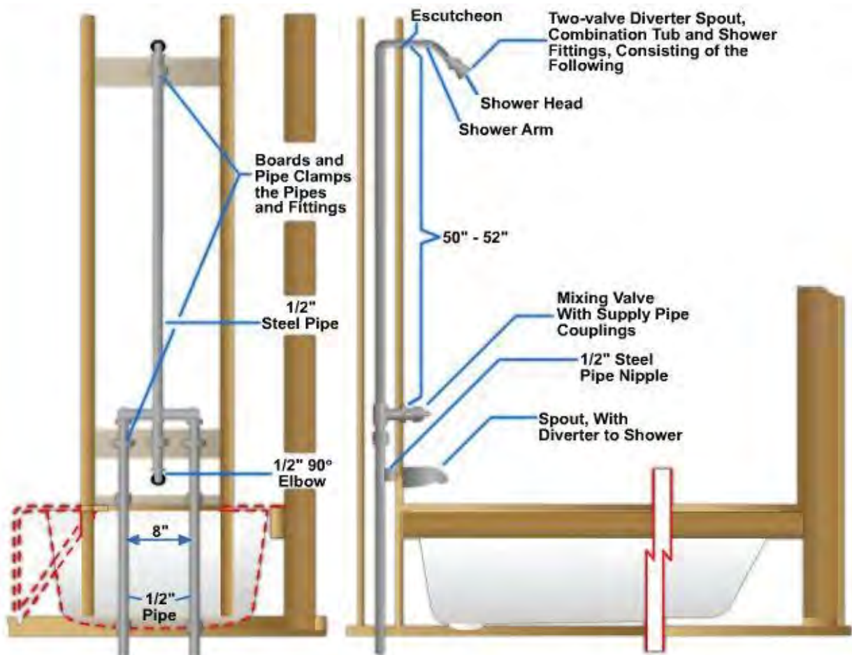
Figure 18 – Bathtub and shower piping combination.
