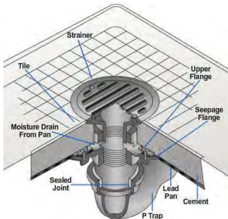
Figure 25 – Cutaway view of a shower pan drain.
