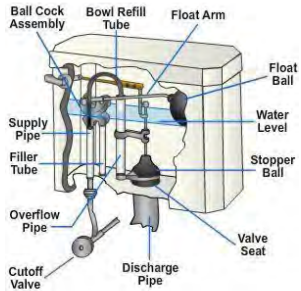
Figure 35 – Water closet flush tank.
