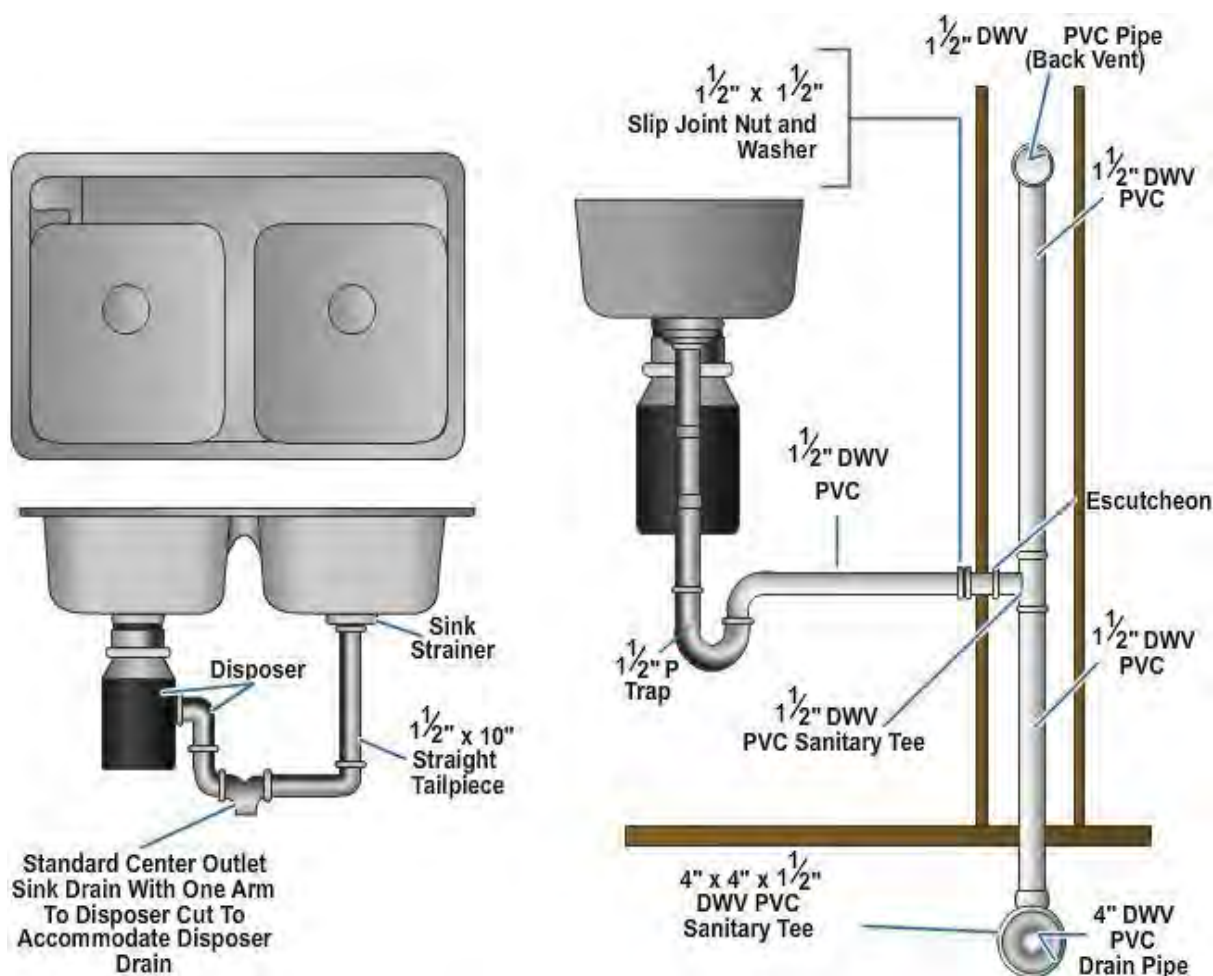
Figure 12 – Kitchen sink waste hookup.
