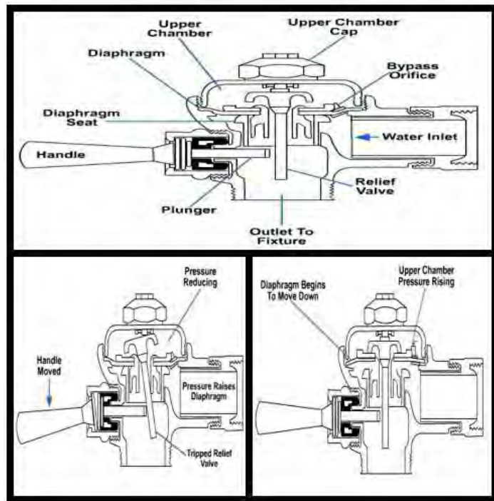
Figure 38 – Operation of diaphragm flushometer.
