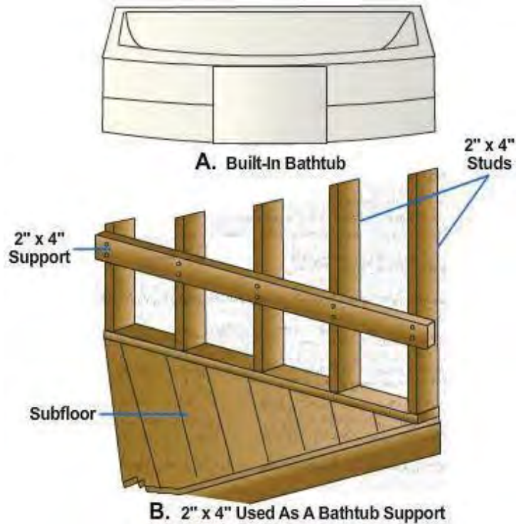
Figure 17 – Bathtub and support.
