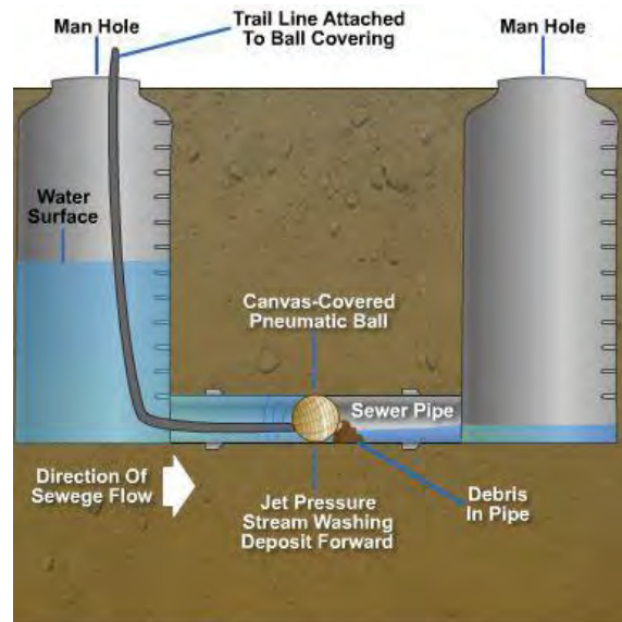
Figure 43 – Ball method of sewer flushing.
