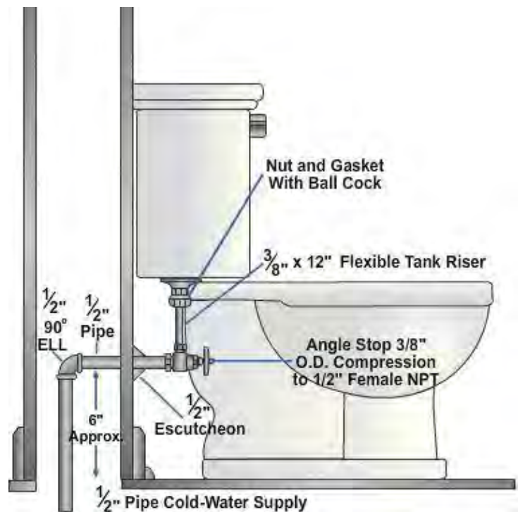
Figure 2 – Water closet (tank type).
