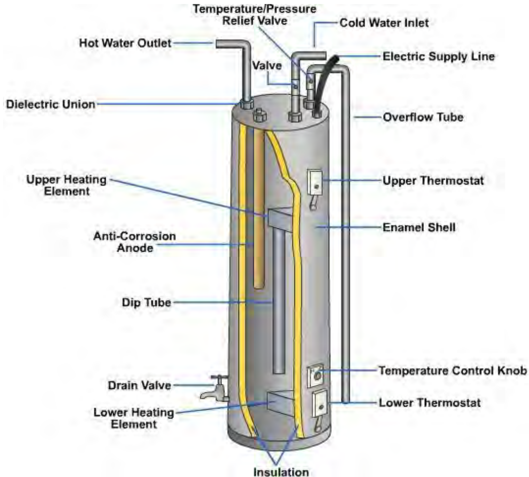
Figure 50 – Electric water heater components.
