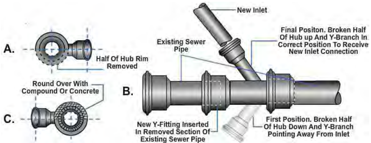
Figure 33 – Adding connections to an outside vitrified clay sewer pipe.
