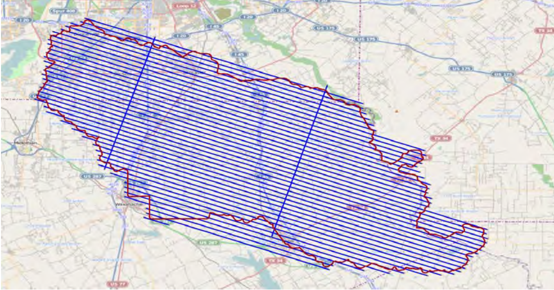
Figure 1-7. LiDAR flight map showing pre-planned flight lines.
