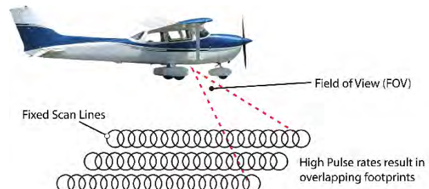
Figure 1-5. Sample scanning pattern produced by a Palmer or elliptical scanning pattern
