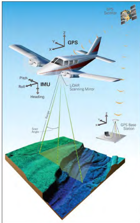
Figure 1-8. Airborne GPS provides x/y/z position of the antenna prior to “lever arm” offset to sensor; IMU provides the roll, pitch and yaw orientation of the LiDAR sensor.
