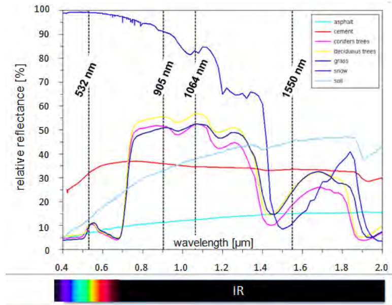
Figure 1-6. Spectral reflectance of various common landscape materials. The common wavelengths used by lidar sensors is also shown. Image courtesy Riegl, GmbH.
