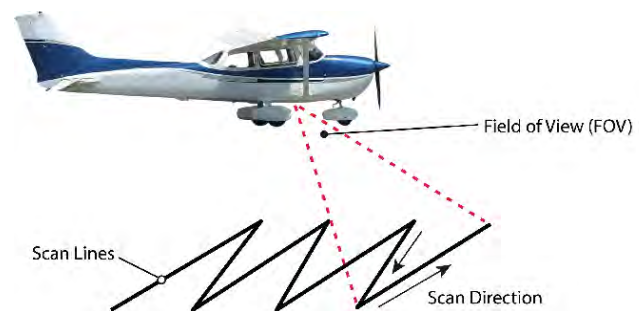
Figure 1-2. Sample scanning pattern produced by an oscillating mirror. The forward look angle of the scanner is for illustrative purposes only. Most scanners operate near nadir-looking scanners when using oscillating mirrors.
