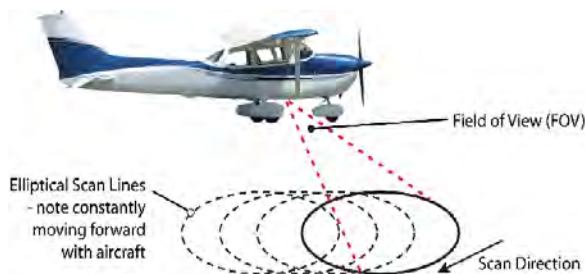
Figure 1-4. Sample scanning pattern produced by a push broom fiber scanning pattern
