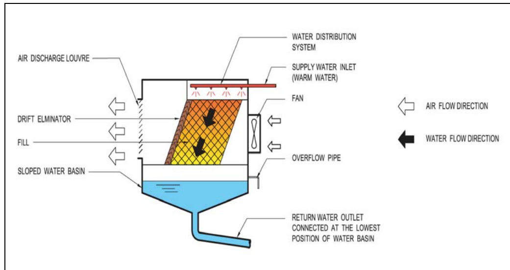
Figure 1.6: Typical configuration of forced draft cross flow cooling tower
