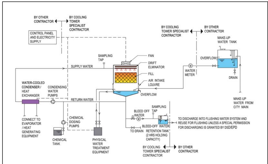
Figure 1.9: Schematic diagram for typical water-cooled air conditioning system
